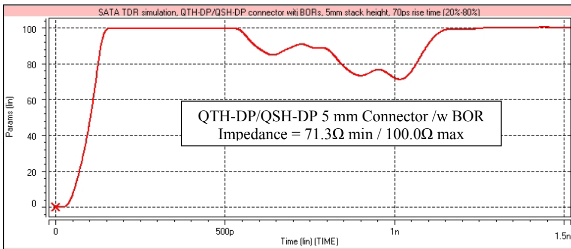
Figure 7 – QTH-DP/QSH-DP Connector with Breakout Routing TDR results
