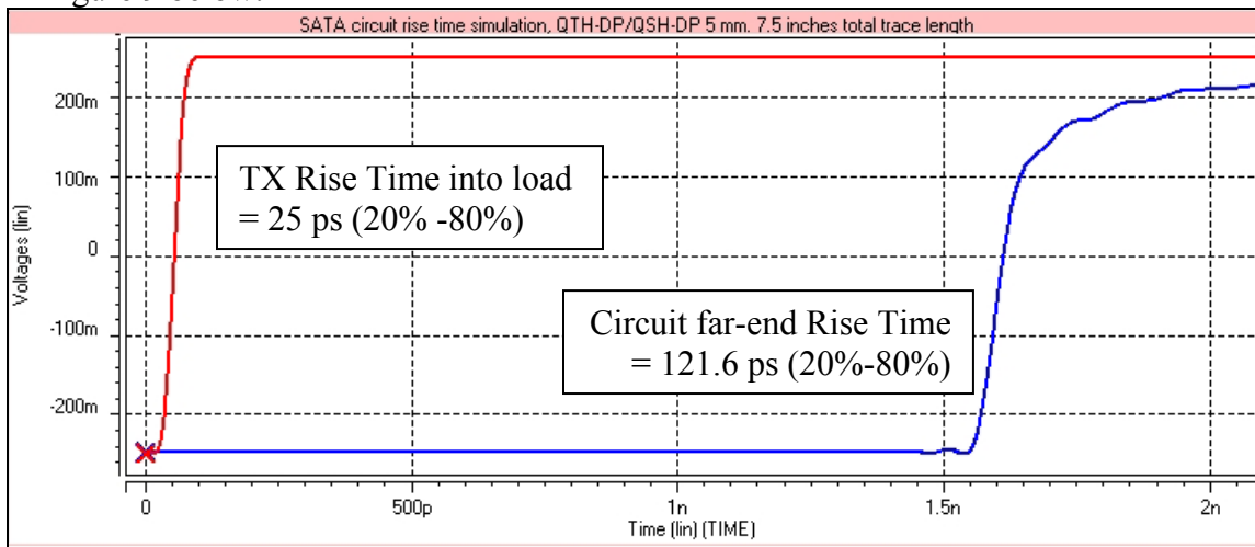
Figure 9 – QTH-DP/QSH-DP Final Inch® circuit rise time results with 7.5 inches total trace length. Red = TX driving compliance load. Blue = Final Inch® circuit probed at the far-end termination.
