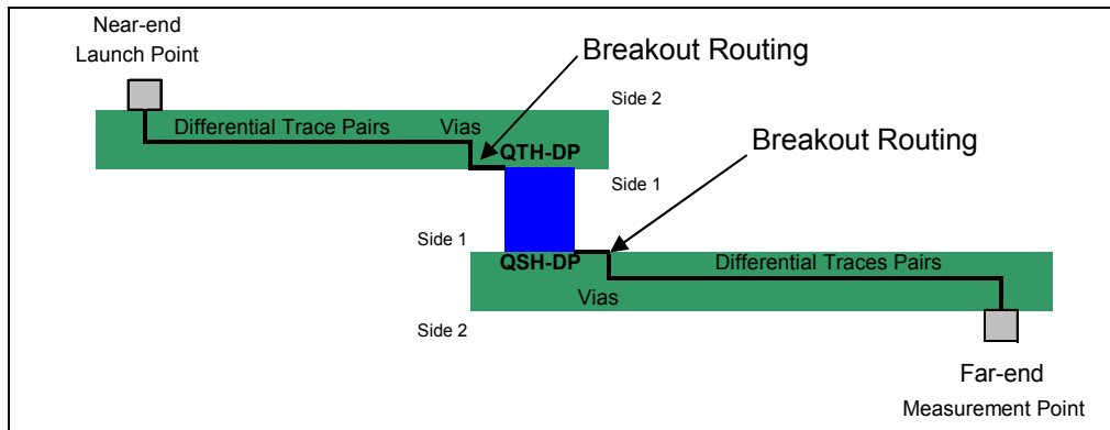
Figure 1 QTH-DP/QSH-DP QPairs® Final Inch® Test Fixture
