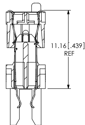
SECTION "E"-"E"
