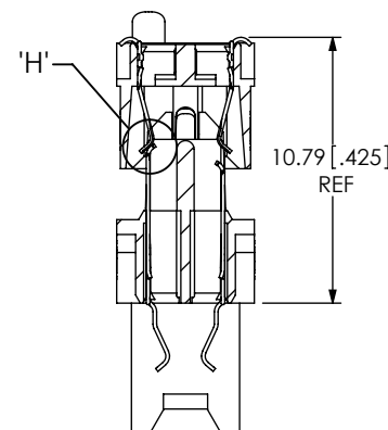
SECTION "F"-"F"
