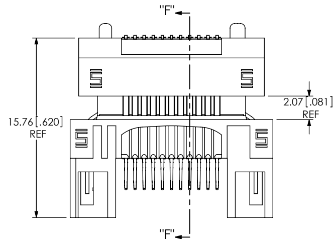
PIN ENGAGING VIEW
