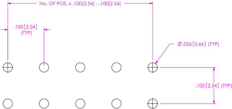
FIG. 1 BBD-105-X-X-X SHOWN (FOR BBD & BDL SERIES ONLY)
