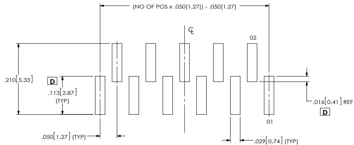
FIG 2 FTS-1XX-XX-X-SV SHOWN ALL DIMENSIONS ARE SYMMETRIC ABOUT THE CENTERLINE
