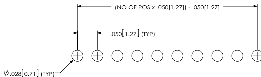
D FIG 1 FTS-1XX-XX-X-S SHOWN ALL DIMENSIONS ARE SYMMETRIC ABOUT THE CENTERLINE
