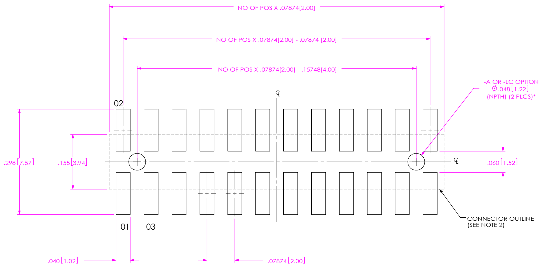
TW-12-XX-X-D-XXX-SM SHOWN
