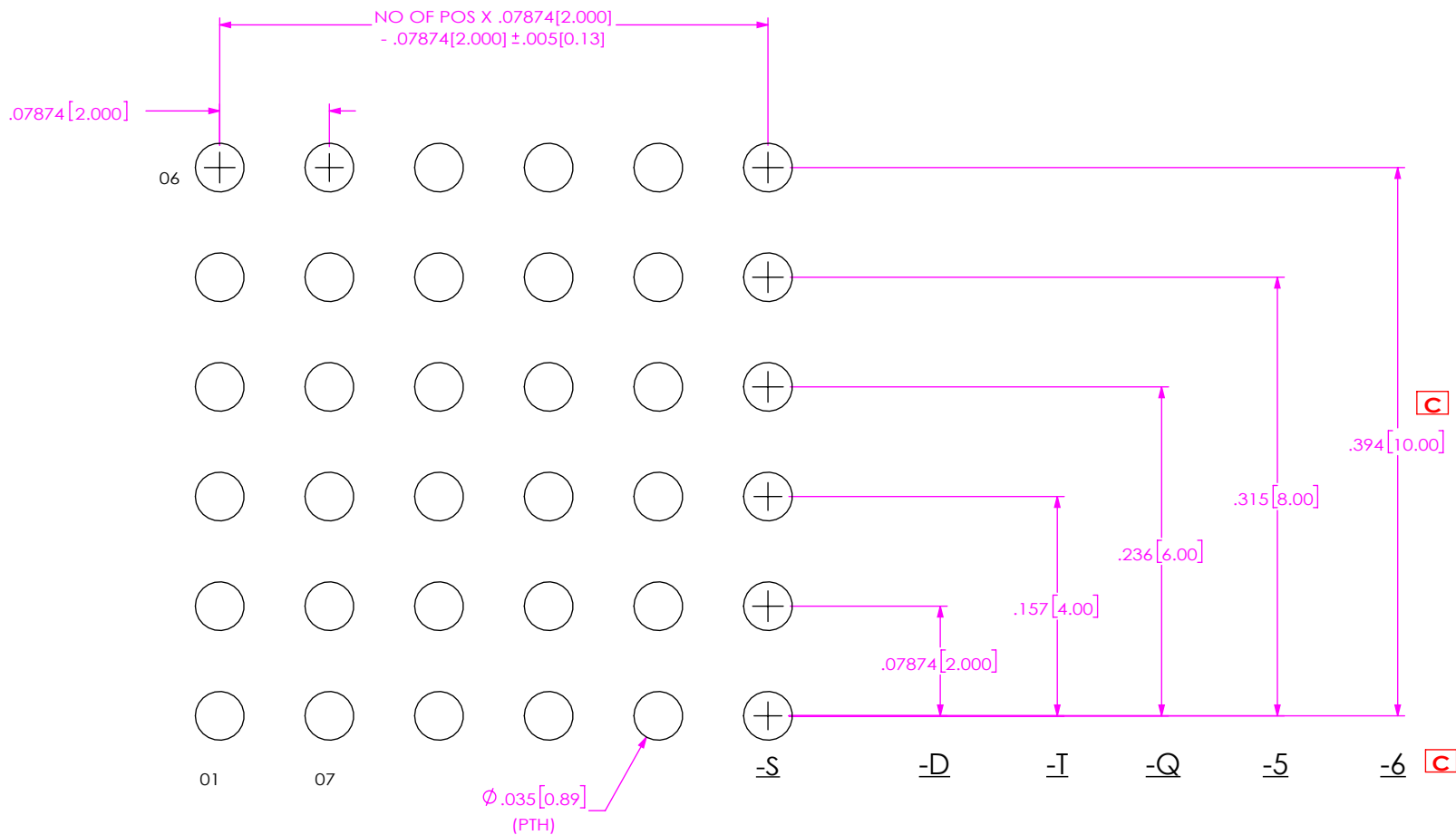
C FIG 1 TW-06-XX-X-6-XXX-XXX SHOWN
